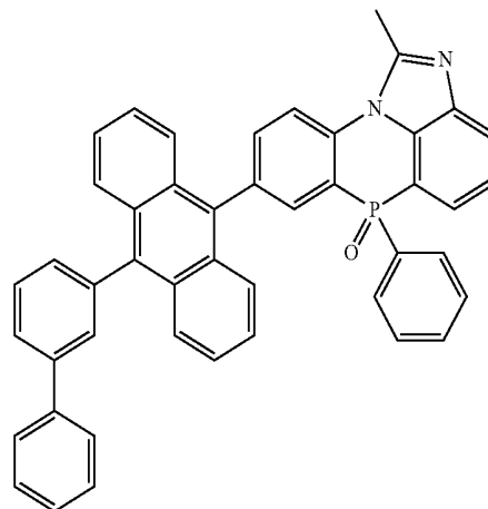
[Chemical Formula 2-2-6]
