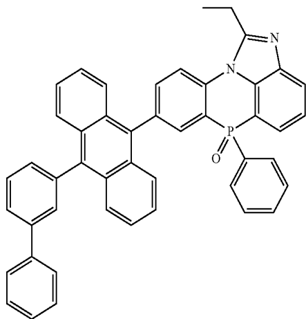
[Chemical Formula 2-3-6]
