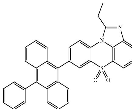
[Chemical Formula 1-3-2]
