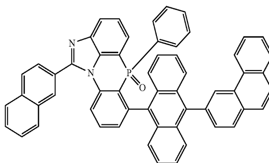
[Chemical Formula 2-6-9]
