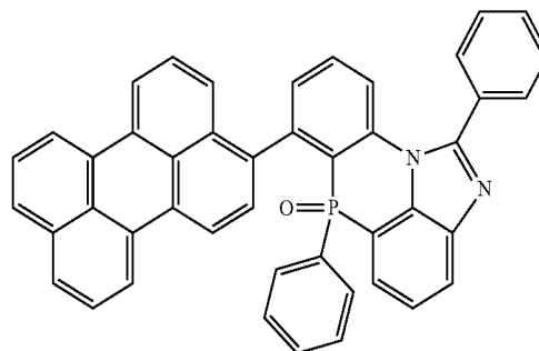
[Chemical Formula 2-6-29]
