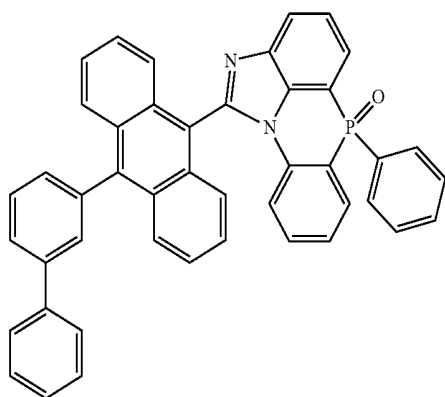
[Chemical Formula 2-5-7]
