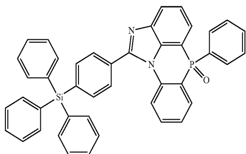
[Chemical Formula 2-2-1]
