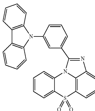
[Chemical Formula 1-1-3]
