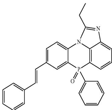
[Chemical Formula 2-3-54]
