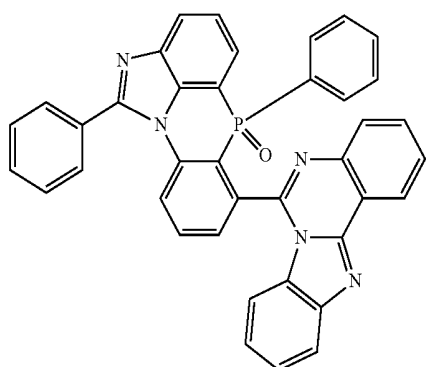
[Chemical Formula 2-6-53]
