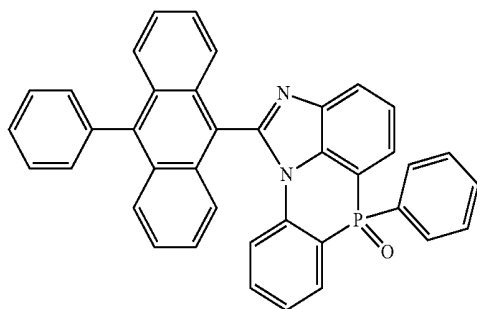
[Chemical Formula 2-5-1]
