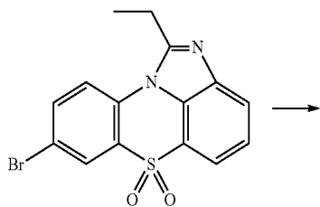
[Compound 2-B]
