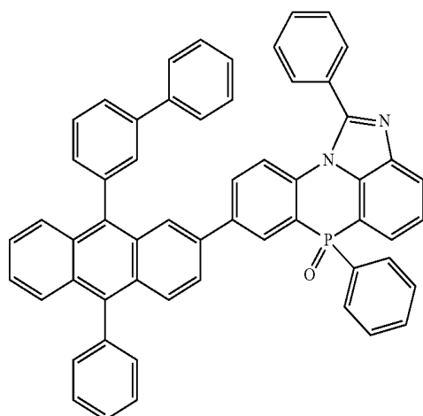
[Chemical Formula 2-4-24]
