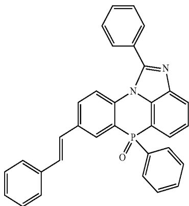
[Chemical Formula 2-4-54]
