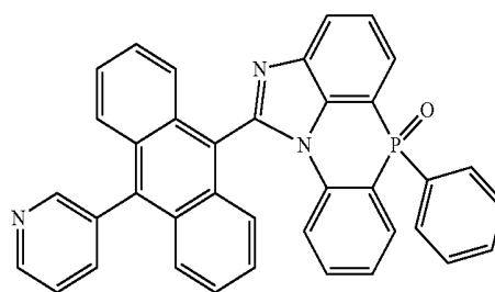
[Chemical Formula 2-5-11]
