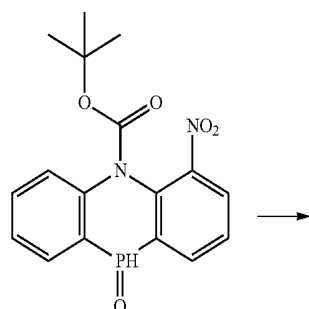
[Compound 2-1-C]
