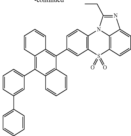
[Chemical Formula 1-3-6]
