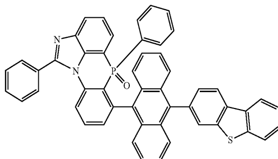
[Chemical Formula 2-6-14]
