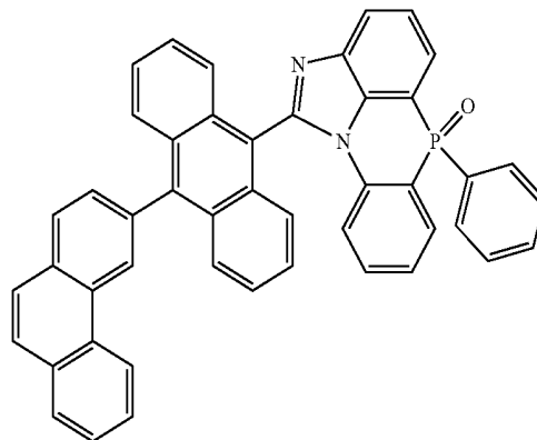
[Chemical Formula 2-5-9]
