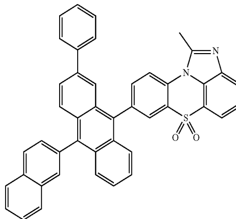
[Chemical Formula 1-2-16]
