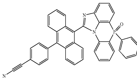
[Chemical Formula 2-5-12]
