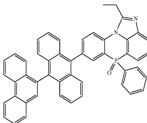
[Chemical Formula 2-3-7]
