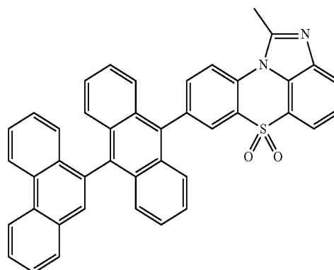
[Chemical Formula 1-2-7]
