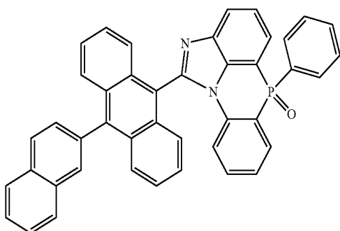
[Chemical Formula 2-5-3]
