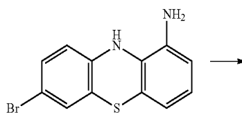
[Compound 1-C]
