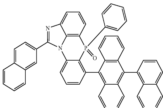
[Chemical Formula 2-6-3]
