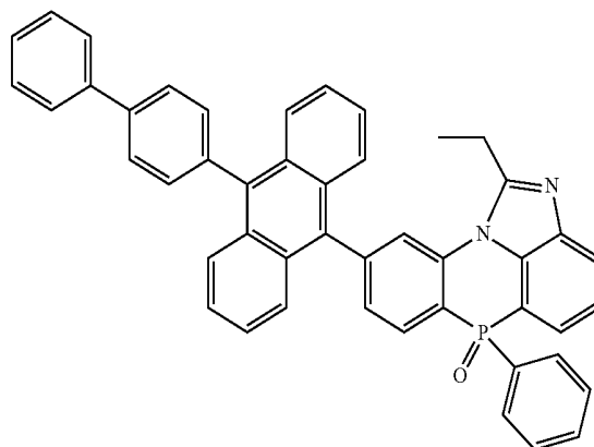
[Chemical Formula 2-7-4]
