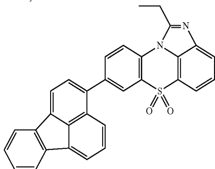
[Chemical Formula 1-3-30]
