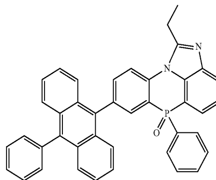
[Chemical Formula 2-3-1]
