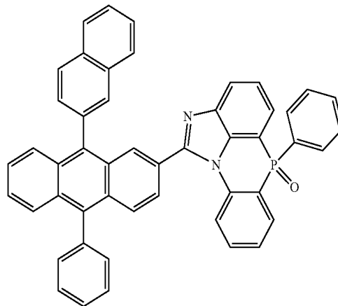
[Chemical Formula 2-5-23]
