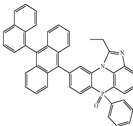
[Chemical Formula 2-7-3]
