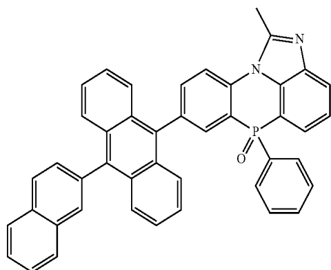
[Chemical Formula 2-2-2]
