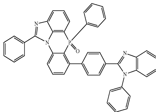
[Chemical Formula 2-6-45]
