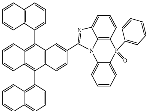
[Chemical Formula 2-5-21]
