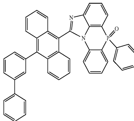
[Chemical Formula 2-5-7]
