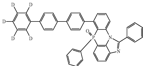
[Chemical Formula 2-6-52]
