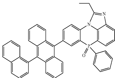
[Chemical Formula 2-3-4]
