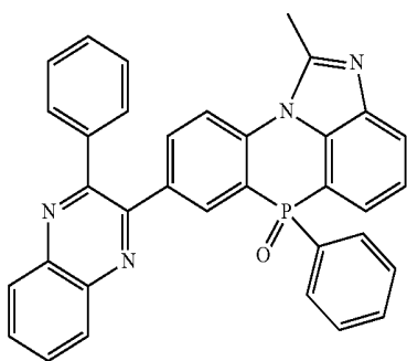
[Chemical Formula 2-2-49]
