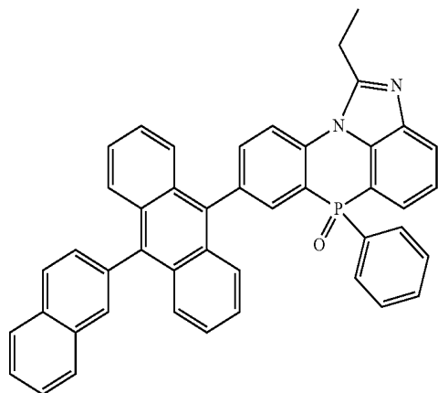
[Chemical Formula 2-3-3]
