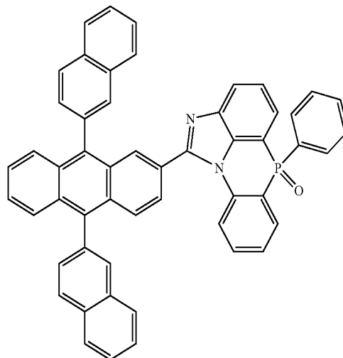
[Chemical Formula 2-5-26]
