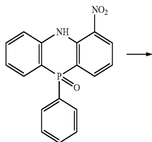
[Compound 2-1-E]
