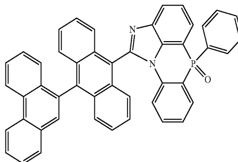
[Chemical Formula 2-5-7]
