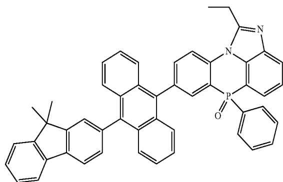
[Chemical Formula 2-3-5]
