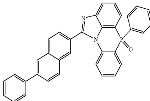
[Chemical Formula 2-5-27]
