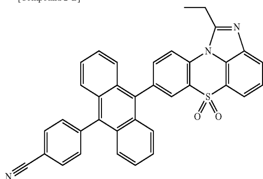
[Chemical Formula 1-3-12]
