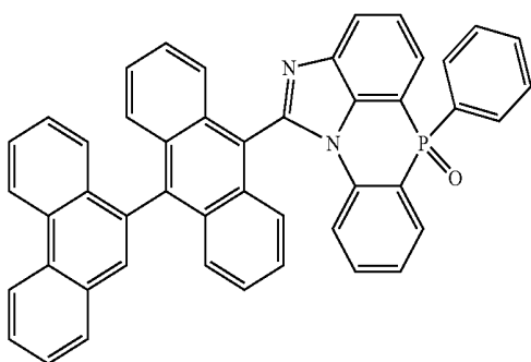
[Chemical Formula 2-5-7]
