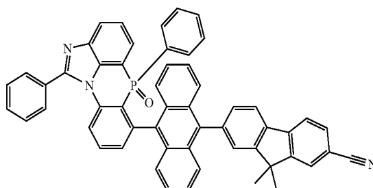
[Chemical Formula 2-6-16]
