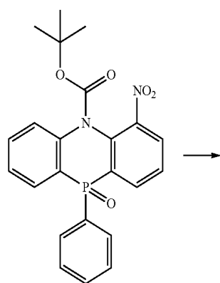
[Compound 2-1-D]
