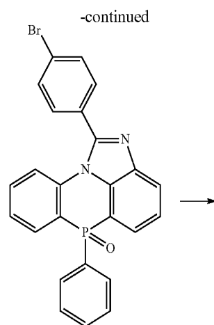
[Compound 2-1-G]
