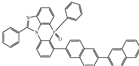
[Chemical Formula 2-6-44]
