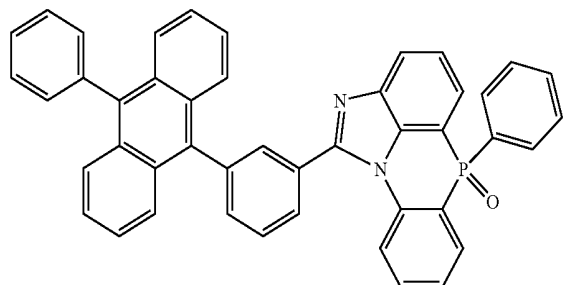
[Chemical Formula 2-5-19]
