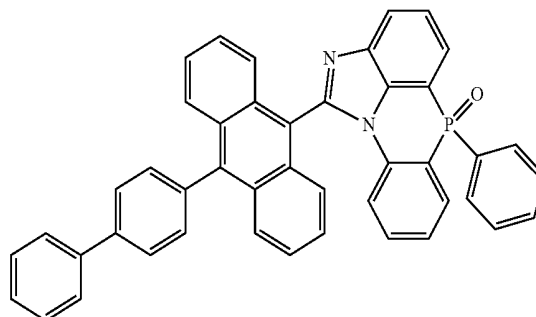
[Chemical Formula 2-5-4]
