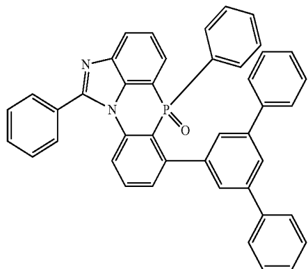
[Chemical Formula 2-6-41]
