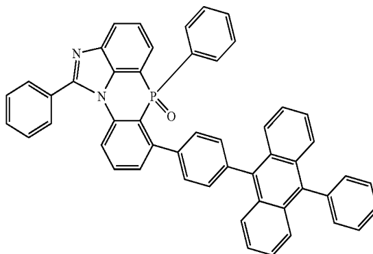
[Chemical Formula 2-6-17]
