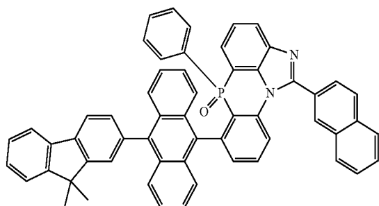
[Chemical Formula 2-6-5]
