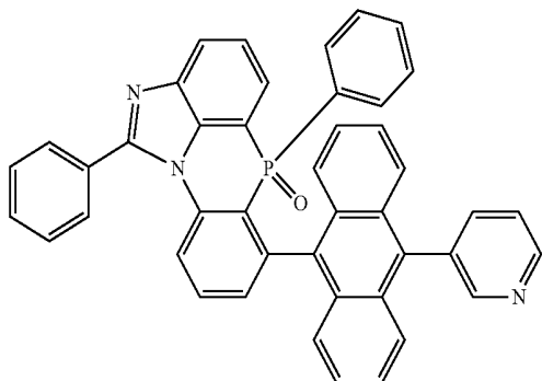
[Chemical Formula 2-6-10]
