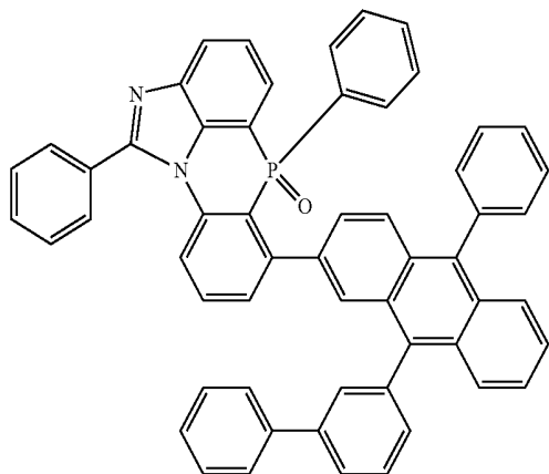
[Chemical Formula 2-6-25]
