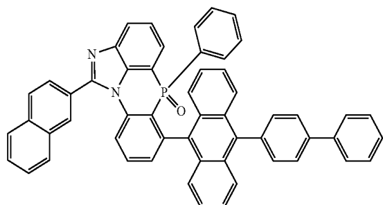
[Chemical Formula 2-6-5]
