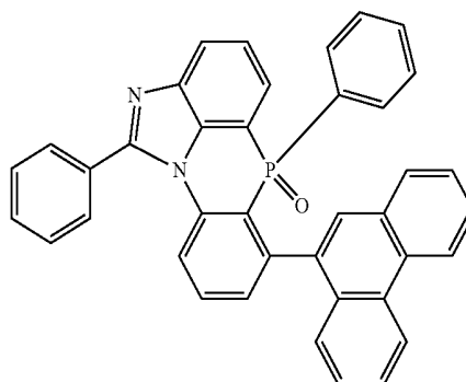
[Chemical Formula 2-6-31]
