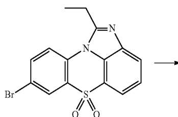
[Compound 2-B]
