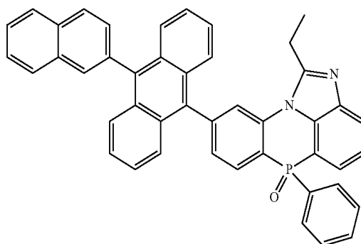
[Chemical Formula 2-7-2]
