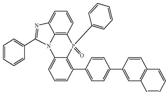
[Chemical Formula 2-6-27]
