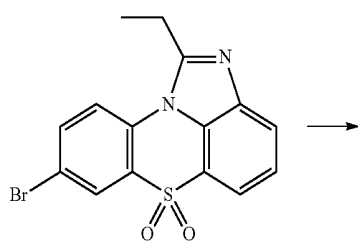
[Compound 2-B]
