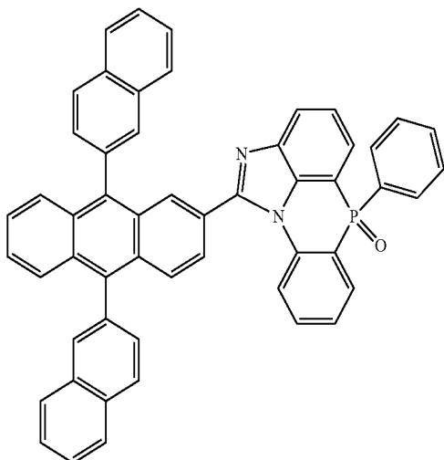
[Chemical Formula 2-5-20]
