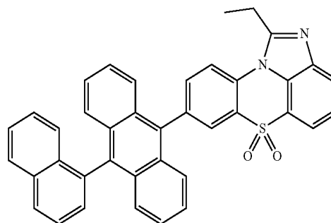
[Chemical Formula 1-3-4]
