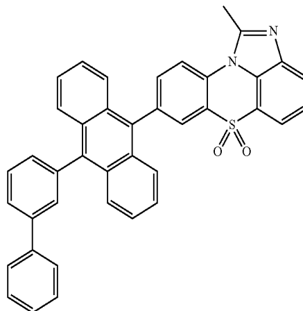
[Chemical Formula 1-2-6]
