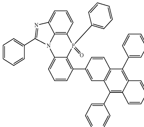
[Chemical Formula 2-6-19]
