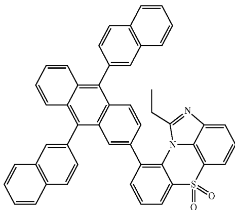
[Chemical Formula 1-8-20]
