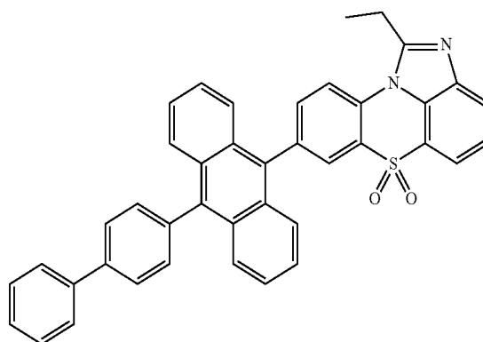
[Chemical Formula 1-3-4]
