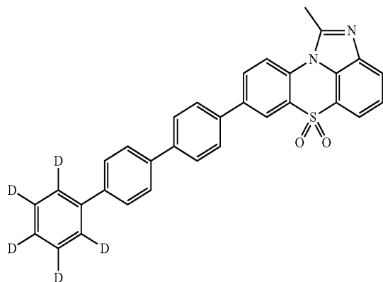
[Chemical Formula 1-2-52]
