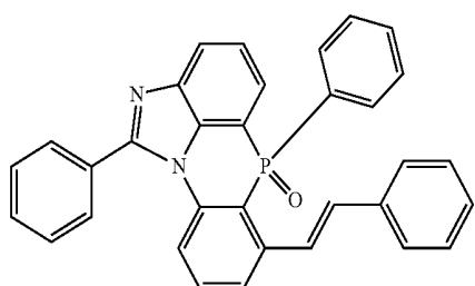
[Chemical Formula 2-7-1]
