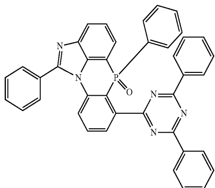
[Chemical Formula 2-6-42]
