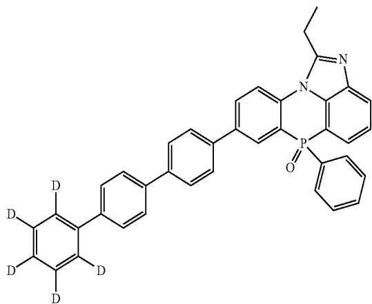
[Chemical Formula 2-3-53]
