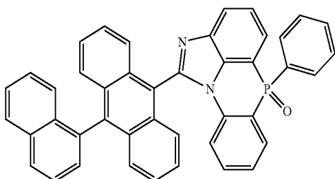
[Chemical Formula 2-5-3]
