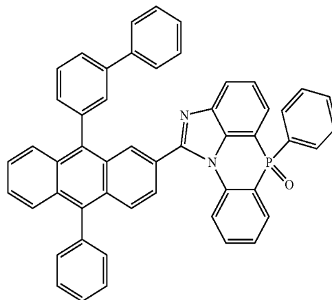
[Chemical Formula 2-5-25]
