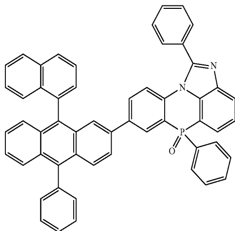
[Chemical Formula 2-4-22]
