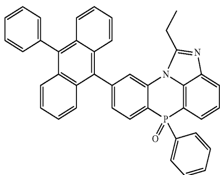
[Chemical Formula 2-7-1]
