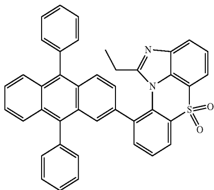
[Chemical Formula 1-8-20]
