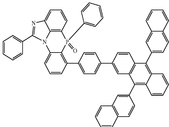
[Chemical Formula 2-6-26]
