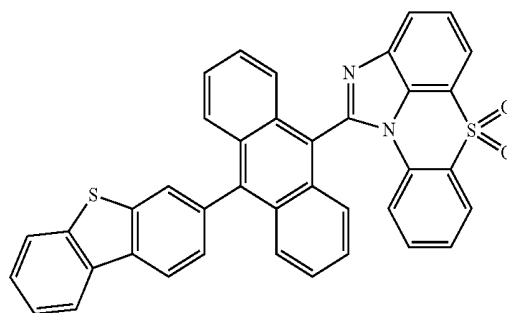
[Chemical Formula 1-5-15]
