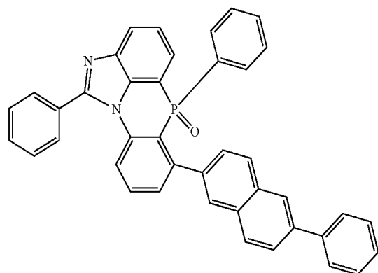
[Chemical Formula 2-6-27]
