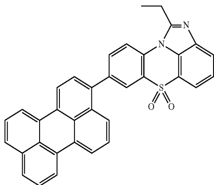
[Chemical Formula 1-3-29]
