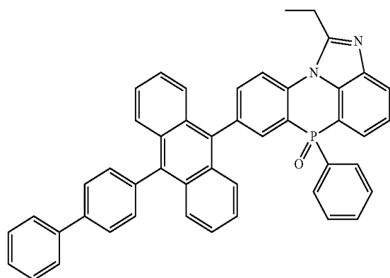
[Chemical Formula 2-3-5]
