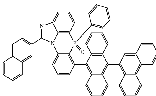
[Chemical Formula 2-6-7]
