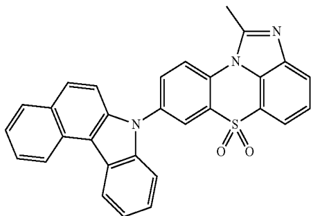
[Chemical Formula 1-2-51]
