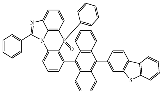
[Chemical Formula 2-6-15]
