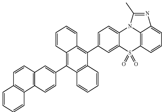
[Chemical Formula 1-2-9]
