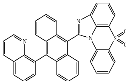
[Chemical Formula 1-5-12]
