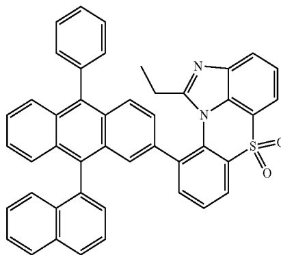
[Chemical Formula 1-8-22]
