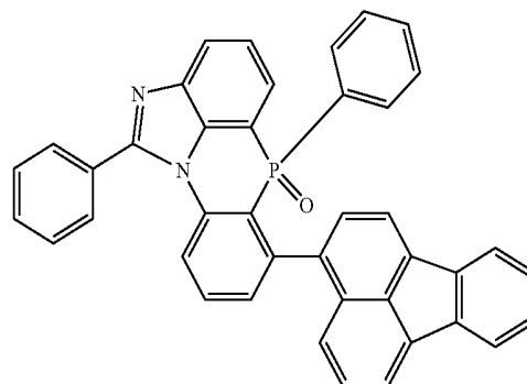
[Chemical Formula 2-6-31]
