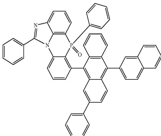
[Chemical Formula 2-6-17]
