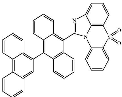
[Chemical Formula 1-5-7]
