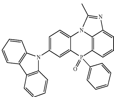
[Chemical Formula 2-2-51]
