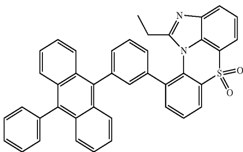
[Chemical Formula 1-8-18]
