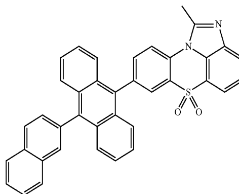
[Chemical Formula 1-2-2]
