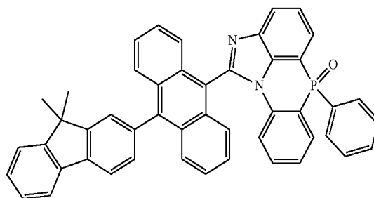
[Chemical Formula 2-5-5]
