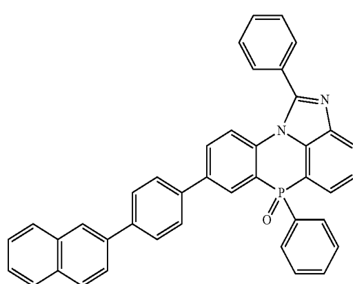
[Chemical Formula 2-4-26]
