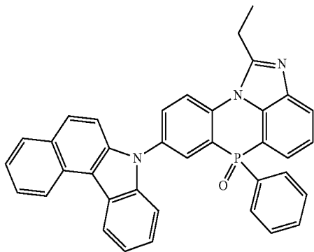
[Chemical Formula 2-3-52]
