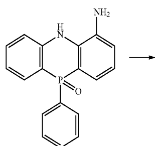
[Compound 2-1-F]
