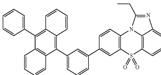
[Chemical Formula 1-3-18]
