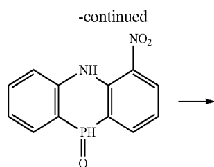
[Compound 2-1-B]
