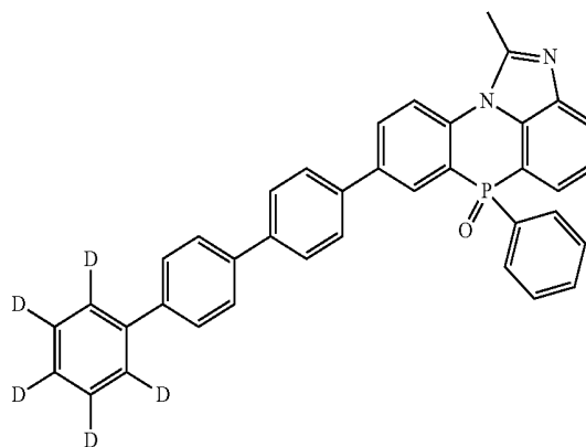
[Chemical Formula 2-2-53]
