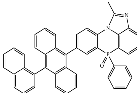
[Chemical Formula 2-2-4]
