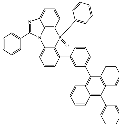
[Chemical Formula 2-6-18]
