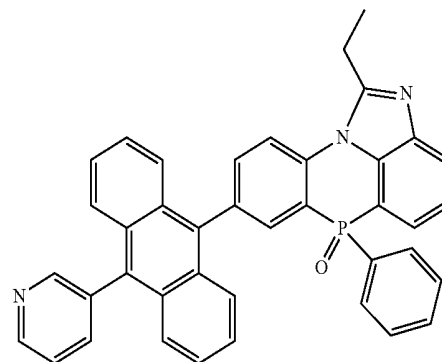
[Chemical Formula 2-3-11]
