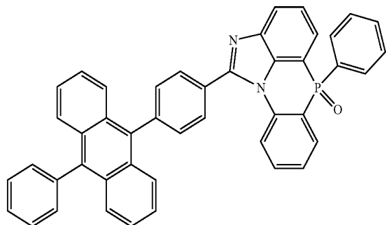
[Chemical Formula 2-5-18]
