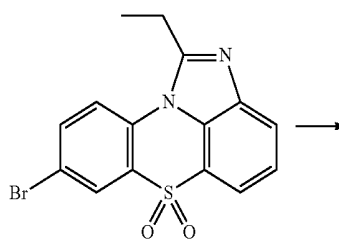
[Compound 2-B]
