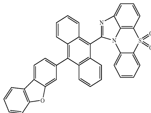
[Chemical Formula 1-5-14]
