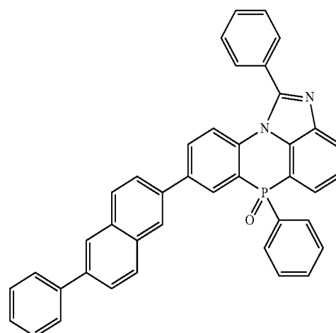
[Chemical Formula 2-4-27]
