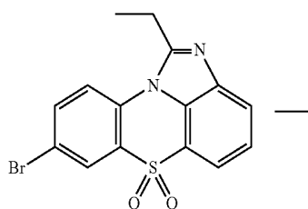
[Compound 2-B]
