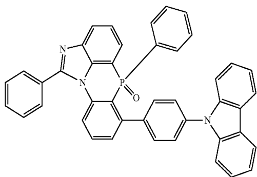
[Chemical 2-6-43]
