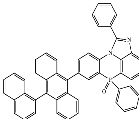
[Chemical Formula 2-4-3]
