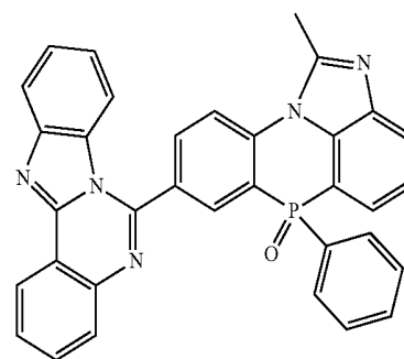
[Chemical Formula 2-2-53]
