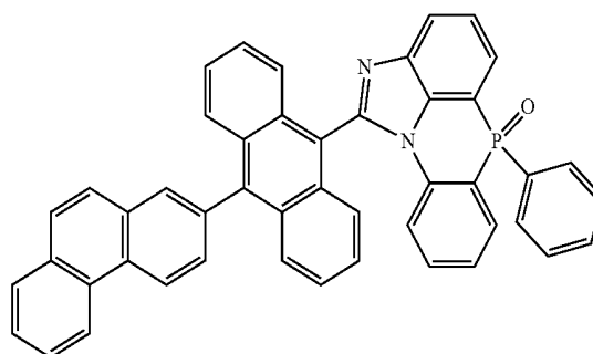
[Chemical Formula 2-5-10]
