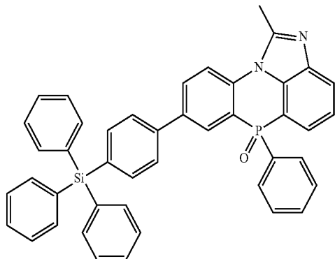
Chemical Formula 2-2-48]
