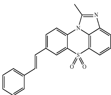
[Chemical Formula 1-2-54]
