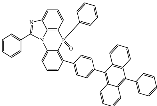
[Chemical Formula 2-6-17]
