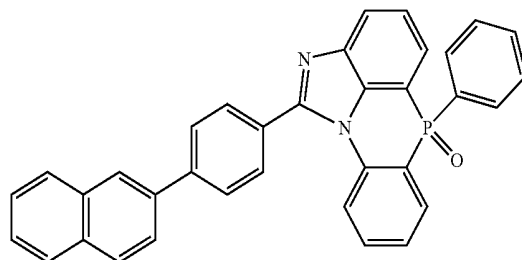
[Chemical Formula 2-5-27]
