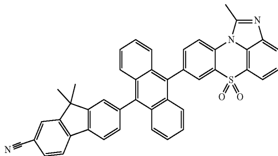
[Chemical Formula 1-2-16]
