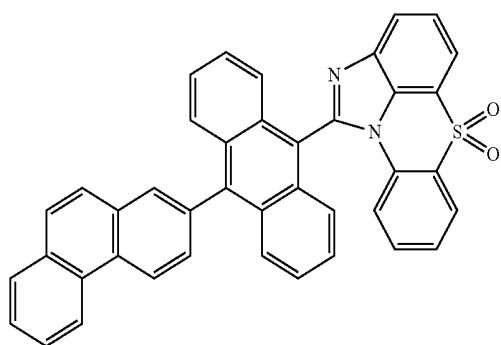
[Chemical Formula 1-5-10]
