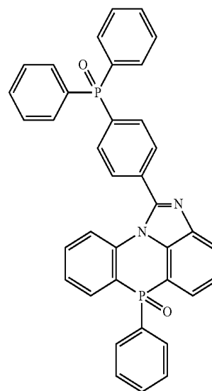
[Chemical Formula 2-12-3]
