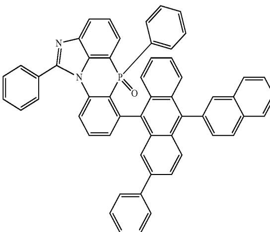
[Chemical Formula 2-6-17]
