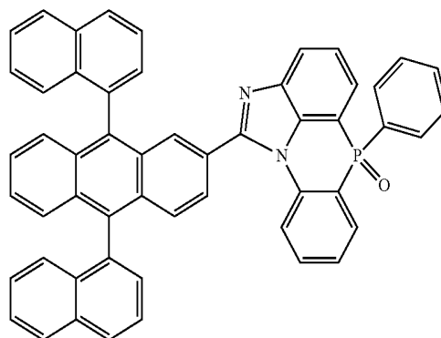
[Chemical Formula 2-5-21]
