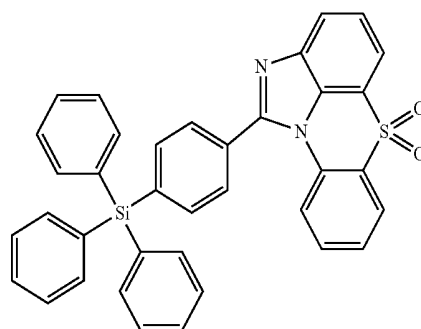
[Chemical Formula 1-2-1]
