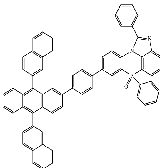
[Chemical Formula 2-4-26]
