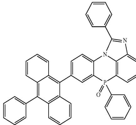
[Chemical Formula 2-4-1]
