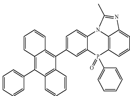
[Chemical Formula 2-2-2]
