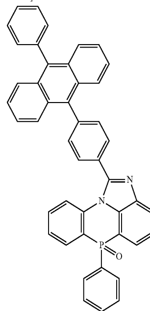
[Chemical Formula 2-5-17]
