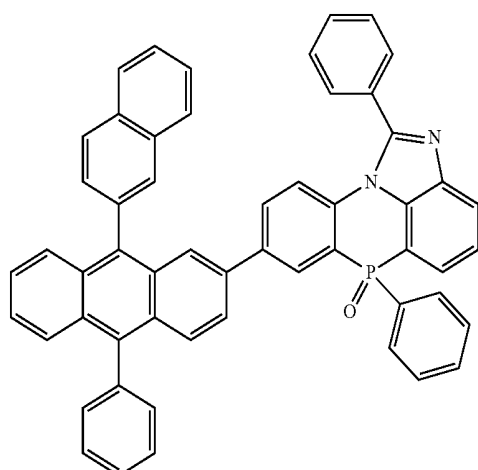
[Chemical Formula 2-4-23]
