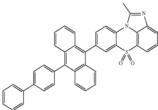
[Chemical Formula 1-2-5]
