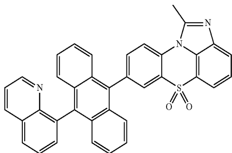
[Chemical Formula 1-2-12]
