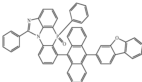
[Chemical Formula 2-6-13]
