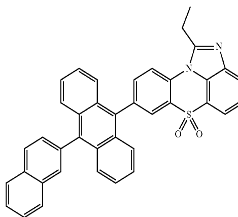
[Chemical Formula 1-3-3]
