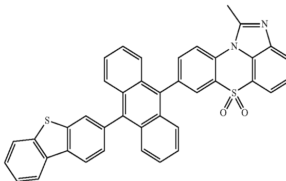
[Chemical Formula 1-2-15]
