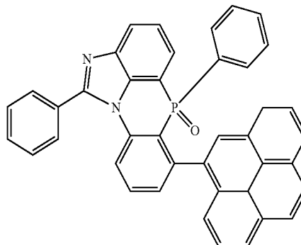
[Chemical Formula 2-6-28]
