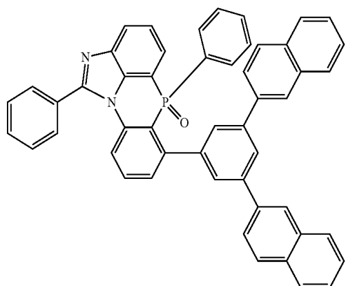
[Chemical 2-6-43]
