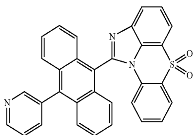
[Chemical Formula 1-5-10]
