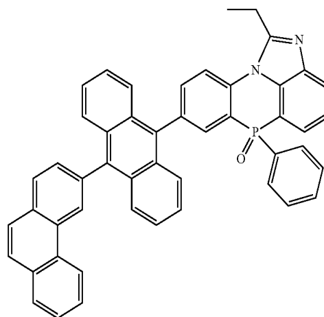
[Chemical Formula 2-3-8]
