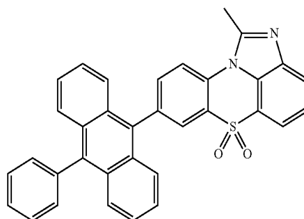
[Chemical Formula 1-2-1]
