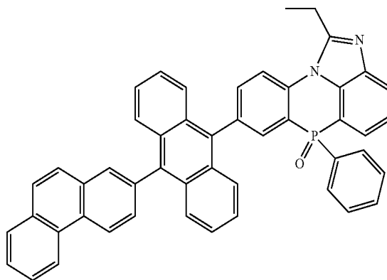
[Chemical Formula 2-3-10]
