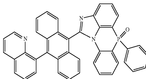
[Chemical Formula 2-5-12]
