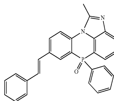
[Chemical Formula 2-3-1]
