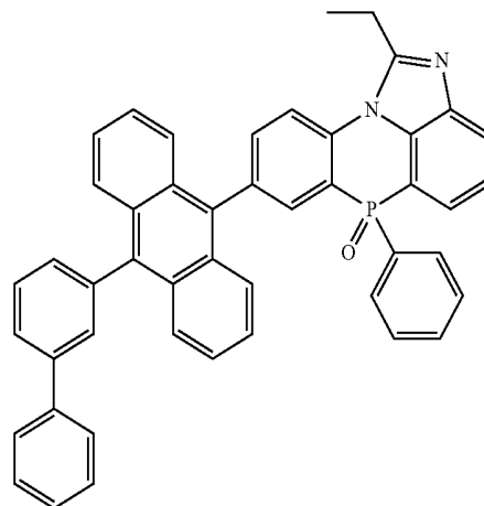
[Chemical Formula 2-3-6]
