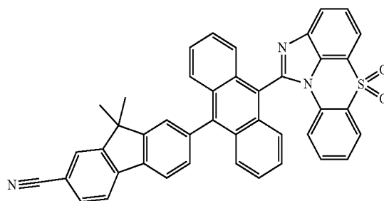
[Chemical Formula 1-5-15]
