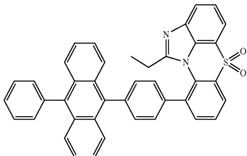
[Chemical Formula 1-8-18]
