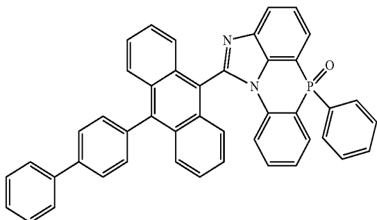
[Chemical Formula 2-5-4]
