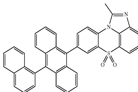
[Chemical Formula 1-2-3]
