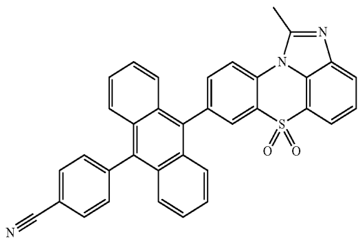
[Chemical Formula 1-2-12]
