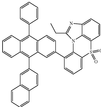
[Chemical Formula 1-8-23]
