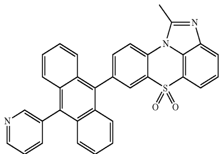
[Chemical Formula 1-2-10]
