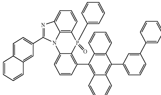
[Chemical Formula 2-6-6]
