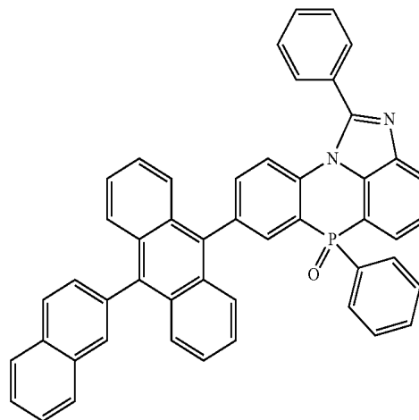
[Chemical Formula 2-4-2]
