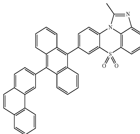
[Chemical Formula 1-2-8]
