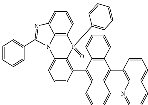
[Chemical Formula 2-6-11]
