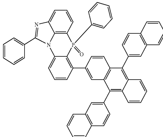
[Chemical Formula 2-6-20]
