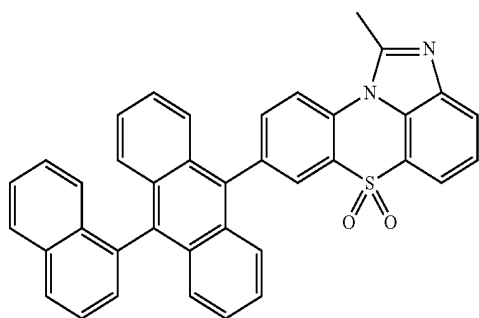
[Chemical Formula 1-2-3]
