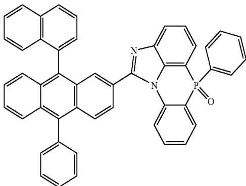
[Chemical Formula 2-5-22]
