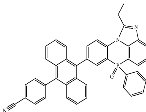
[Chemical Formula 2-3-12]
