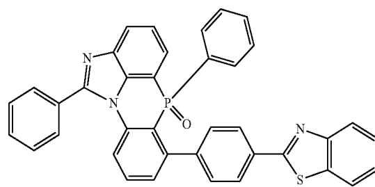
[Chemical Formula 2-6-47]
