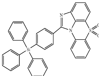
[Chemical Formula 1-2-1]
