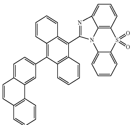
[Chemical Formula 1-5-9]
