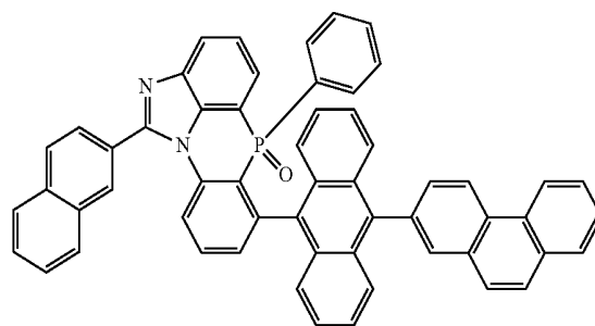
[Chemical Formula 2-6-9]
