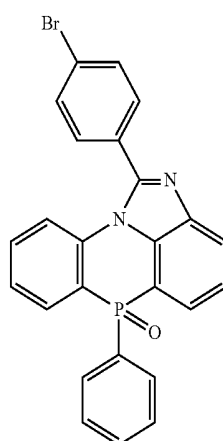
[Compound 2-1-G]
