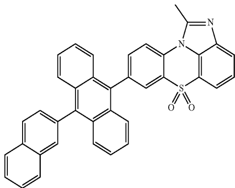
[Chemical Formula 1-2-3]
