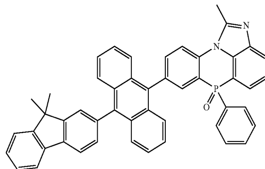
[Chemical Formula 2-2-6]
