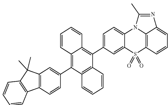
[Chemical Formula 1-2-5]
