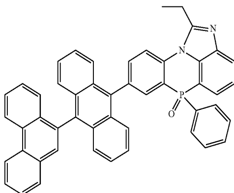
[Chemical Formula 2-3-7]
