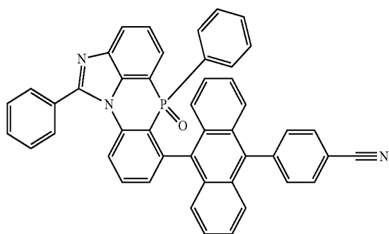
[Chemical Formula 2-6-13]
