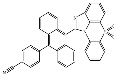
[Chemical Formula 1-5-13]
